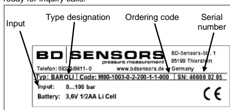
Fig. 1 manufacturing label
